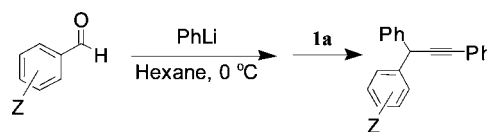
Scheme 3. A Tandem Reaction to Internal Alkynes
